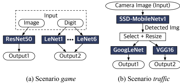
Figure 12: Two multi-model applications: game and traffic .
