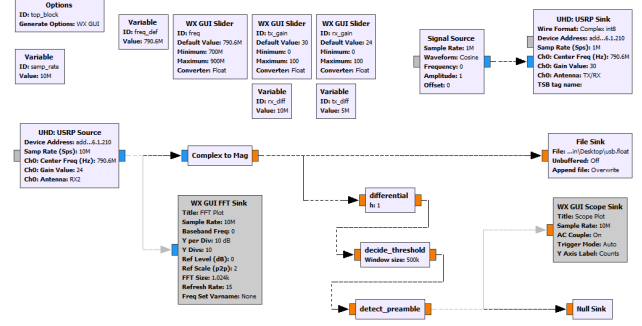
Figure 10: Composition of GNU Radio blocks used for decoding the observed radio wave signals.
