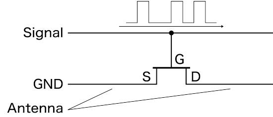
Figure 1: A RF retroreflector that includes a FET chip and a dipole antenna. An internal signal is applied to the gate of FET.
