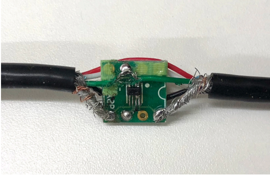
Figure 8: A photo of RFRA embedded into a USB cable.
