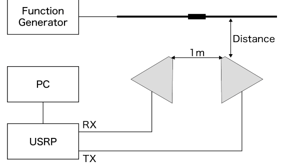
Figure 4: Experimental setup (overview).
