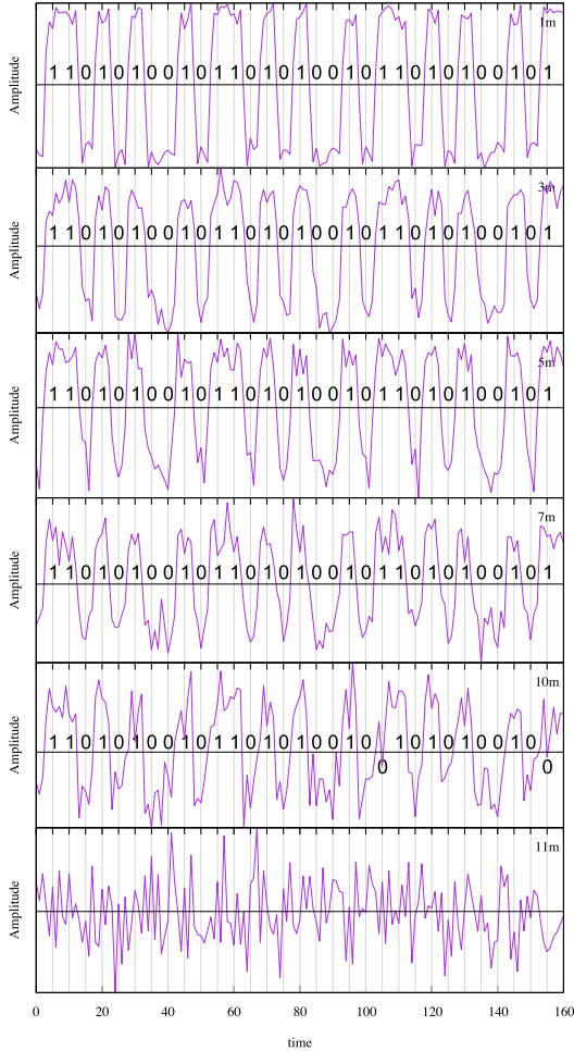
Figure 5: Measured signals under different distances between the attacker and the target.
