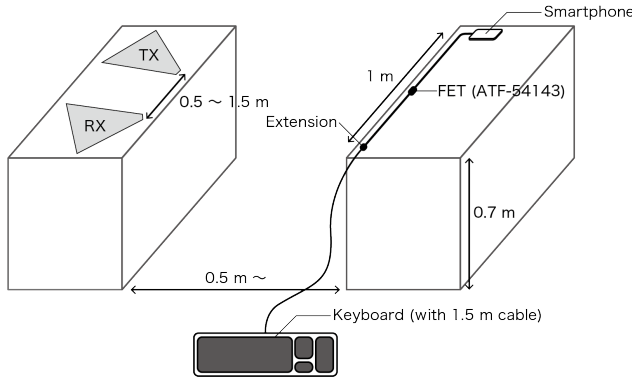
Figure 9: Experiment setup.
