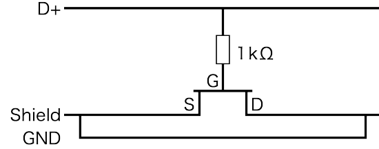
Figure 7: A circuit of RFRA embedded into a USB cable.
