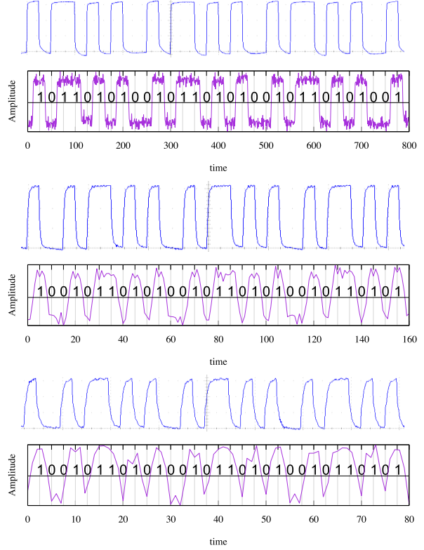
Figure 6: Measured waveforms for the target signals with the frequencies of 1 Mbps (top), 5 Mbps (middle), and 10 Mbps (bottom). The upper part of each figure is a waveform measured by oscilloscope.
