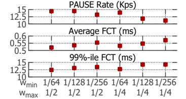
Figure 13: Performance of PCN with different w_{\min} and w_{\max} .
