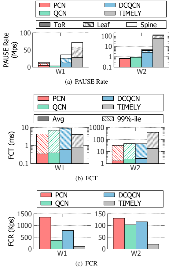
Figure 14: Performance for realistic workloads.
