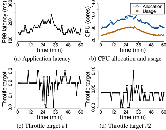
Figure 6: Measurements of Social-Network under diurnal workload. Figure (a) and (b) show the latency and CPU statistics achieved by Autothrottle. Figure (c) and (d) demonstrate how Tower adjusts performance targets in response to the time-varying workload, for the two CPU usage groups (§A.3).
