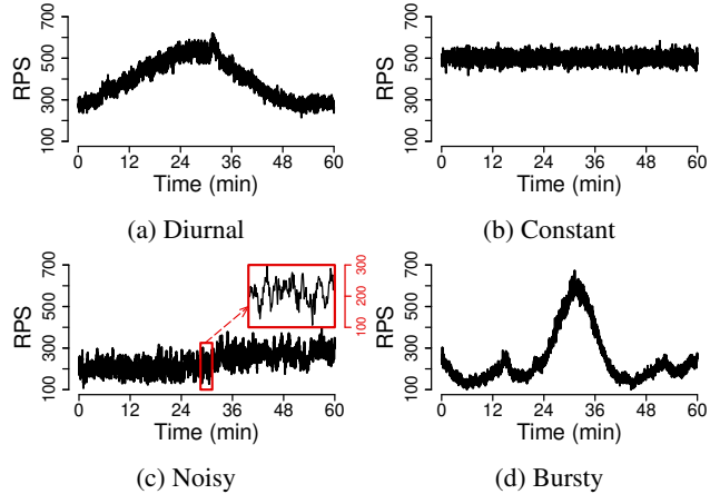
Figure 3: Our workload traces capture common patterns of RPS (requests per second) on an hourly basis. These patterns have been observed in real-world scenarios: Puffer streaming requests [57], Google cluster usage [55], and Twitter tweets [9]. We also recorded a full 21-day workload trace from a global cloud provider for long-term evaluation. We scale these traces accordingly for each benchmark application to saturate the cluster (§A.5).
