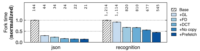
Figure 18. Effects of optimizations applied by MITOSIS.
