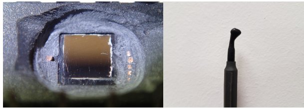
(a) Target 8-bit microcontroller mechanically decapsulated (b) Langer RF-U 5-2 Near Field Electromagnetic passive Probe
