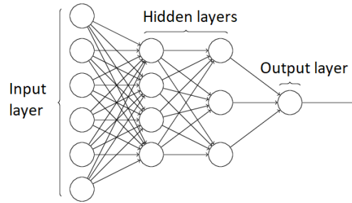
Figure 1: Multilayer perceptron.
