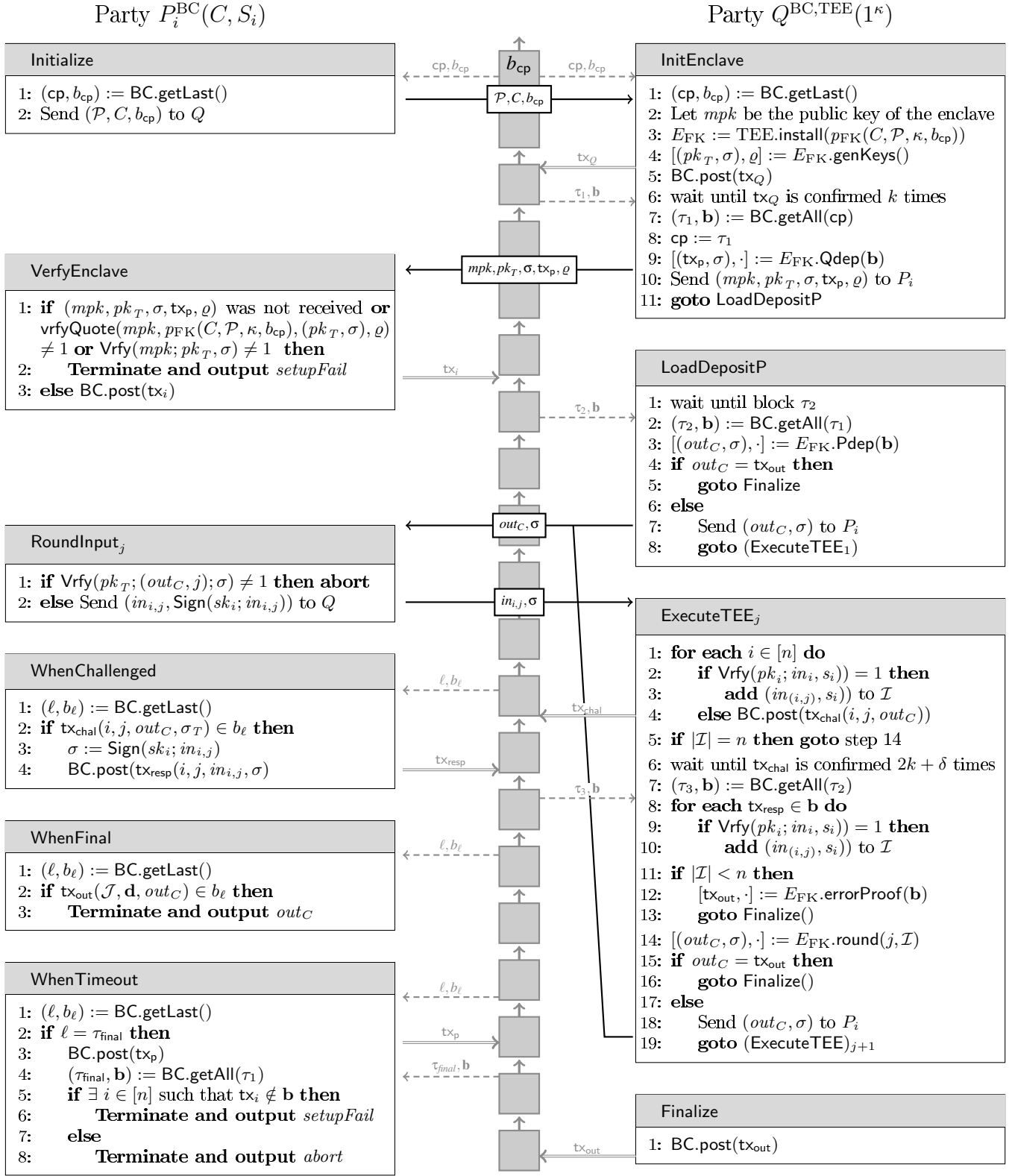
Figure 2: Protocol \pi_{FASTKITEN} . Direct black arrows indicate communication between the parties and Q , gray dashed arrows indicate reading from the blockchain and gray double arrows posting on the blockchain.
