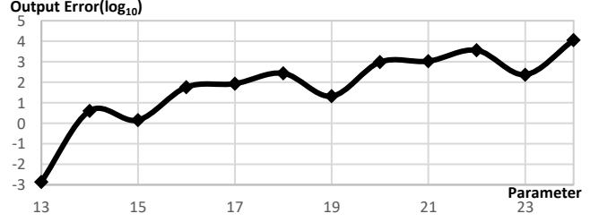
Figure 5: The input scale parameter of EVA leads to an arbitrary variation in the output error in LeNet-5.
