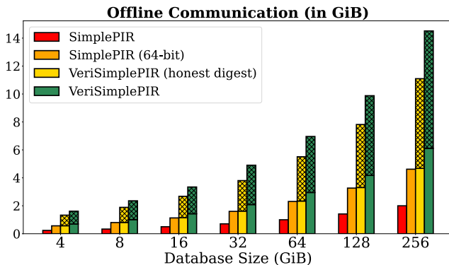
Figure 8: Offline communication of SimplePIR and preprocessed VeriSimplePIR for databases of various sizes. The hatched portions in the VeriSimplePIR columns represent the communication that is not stored once the precomputation is finished. The unhatched portion represents the data that the client must store locally throughout the protocol (including the online phase).
