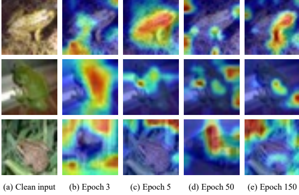
Figure 3: The attention maps on training epochs 3, 5, 50, and 150. The accuracy of the model on CIFAR-10 is 53.74%, 64.49%, 86.76%, and 94.92%, respectively.
