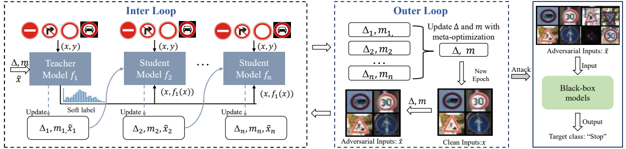
Figure 2: Overview of CleanSheet. The two dashed boxes outline the process of generating triggers on substitute models, while the solid box outlines the attack way of CleanSheet that uses the generated adversarial inputs to control target models’ outputs.
