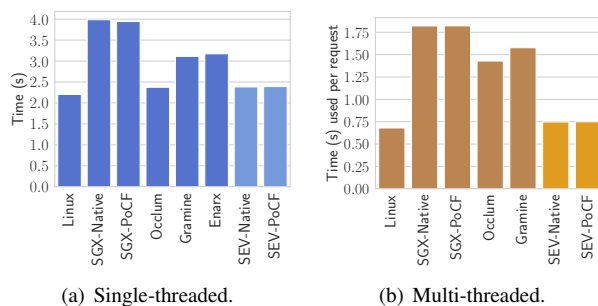
Figure 8: Macrobenchmark: FASTA execution time.
