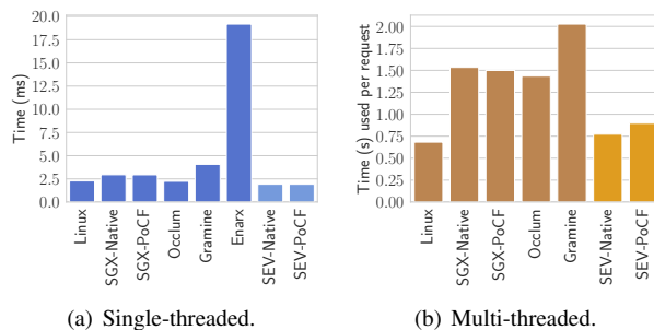
Figure 7: Macrobenchmark: AI inference execution time.
