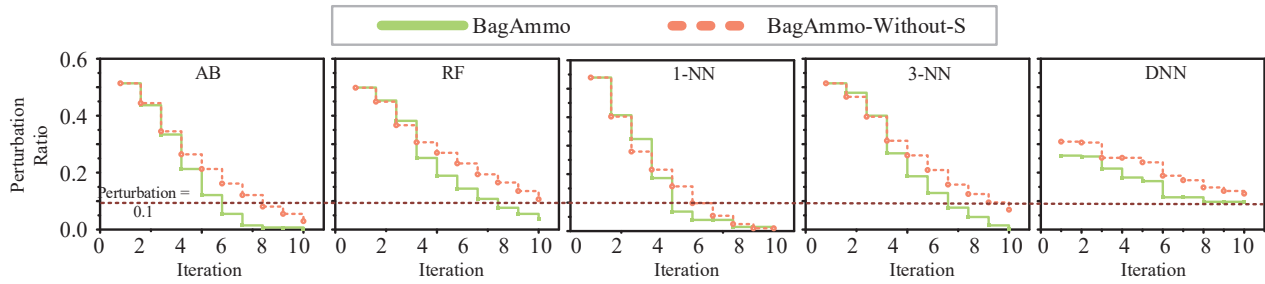
Figure 12: With substitute model vs. without substitute model.
