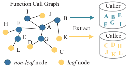
Figure 4: Selecting callers and callees from an FCG.
