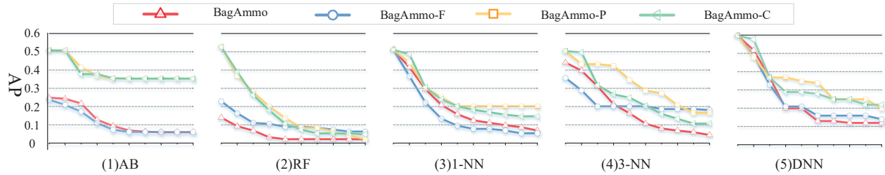
Figure 10: Multi-population vs. single-population.
