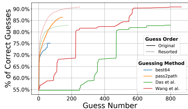
Figure 6: Comparison of the credential tweaking approaches.
