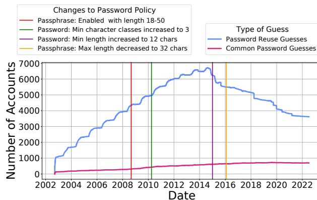
Figure 2: At the time indicated on the x-axis, the number of accounts actively using a password we correctly guessed.
