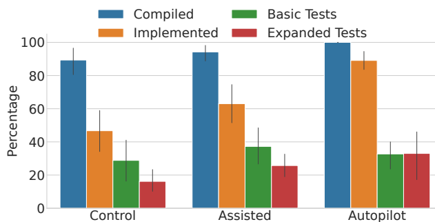
Figure 7: Functionality for each group. Each group has to implement 11 functions and 11 basic tests. We had 43 expanded tests. We show per group, the average % of functions Implemented , regardless of whether they compiled or not, the average % of those functions that Compiled , the average % of each group that passes the 11 Basic Tests and the average % that passes the 43 Expanded Tests from each group.
