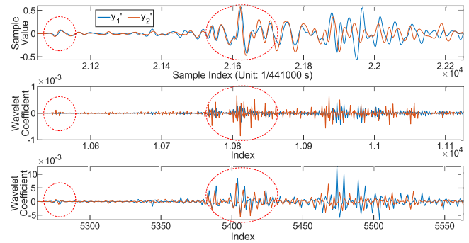
Figure 2: Top: Keystroke signals aligned based on cross-correlation results. Middle: Level-1 wavelet coefficients. Bottom: Level-2 wavelet coefficients. We can perceive the misalignments in the signals especially their transient parts (in red circles) more clearly from the wavelet decomposed signals. Even in the same level of coefficient, the other parts of the recorded signals ( y_1 and y_2 ) differ significantly. These components will result in the miscalculation of the time delay.
